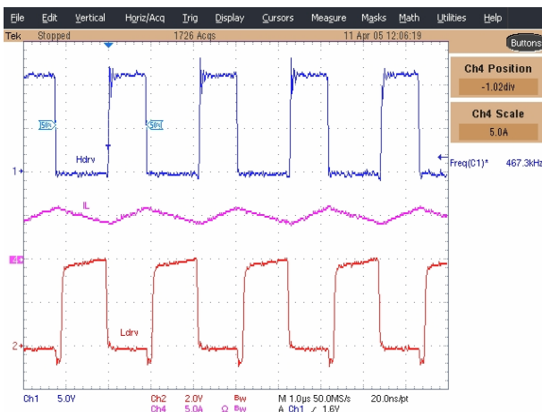
Figure 6 - Gates waveforms Ch1: Hdrv, Ch2: Ldrv, Ch3: Inductor Current I_{Load}=5A
